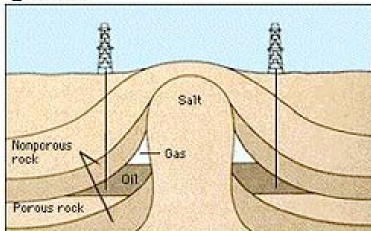
Salt dome
