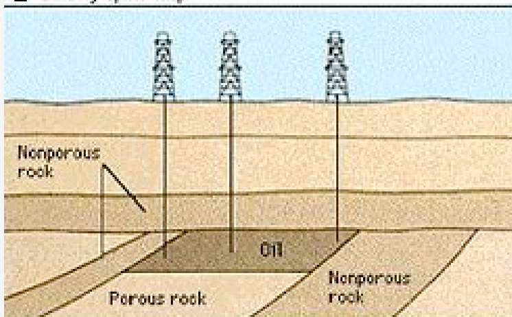
Stratigraphic trap
